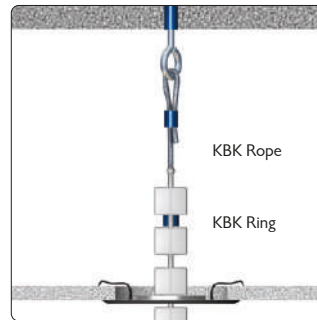
Mounting with tension rope on raw ceiling
