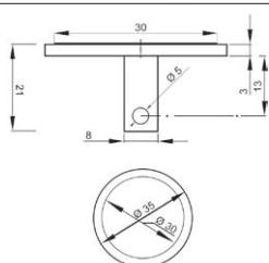
KBK Glue, KBK Steel, KBK Ring, Glass table
