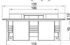
KBK Outlet Z30 for guiding single cables
