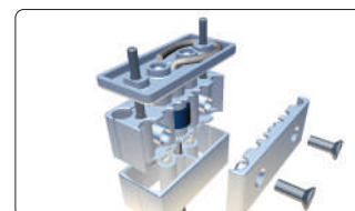
Clip fixation of tension rope KBK Rope
