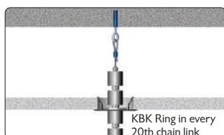
Ceiling-suspension with KBK Rope & KBK Ring
