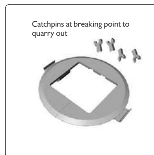
KBK Cover without application of force into the ceiling
