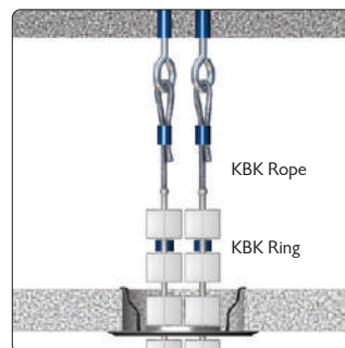
Mounting 2x KBK Cube on raw ceiling
