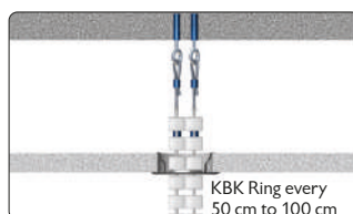
Ceiling suspension with KBK Rope & KBK Ring
